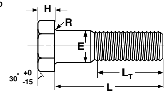
Rolled Thread
