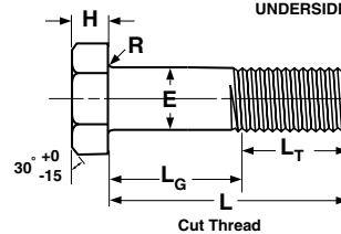
Cut Thread
